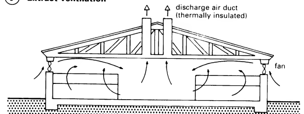
⑩ Pressurised ventilation
